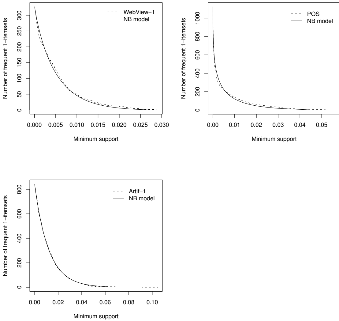
Figure 2: Actual versus predicted number of frequent items by minimum support.
