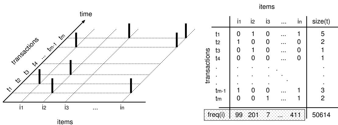
Figure 1: Representation of an example database as a sequence of transactions (to the left) and the incidence matrix with the resulting frequencies of the single items (to the right).
