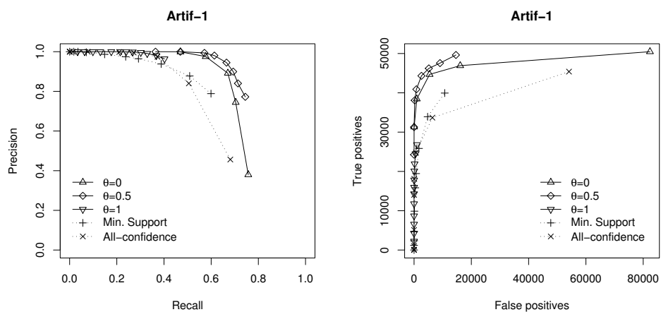
Figure 11: Performance of the algorithm on Artif-1 using 20,000 transactions.
