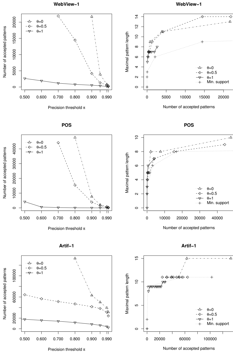
Figure 9: Comparison of different settings for the pattern generation on three data sets.
