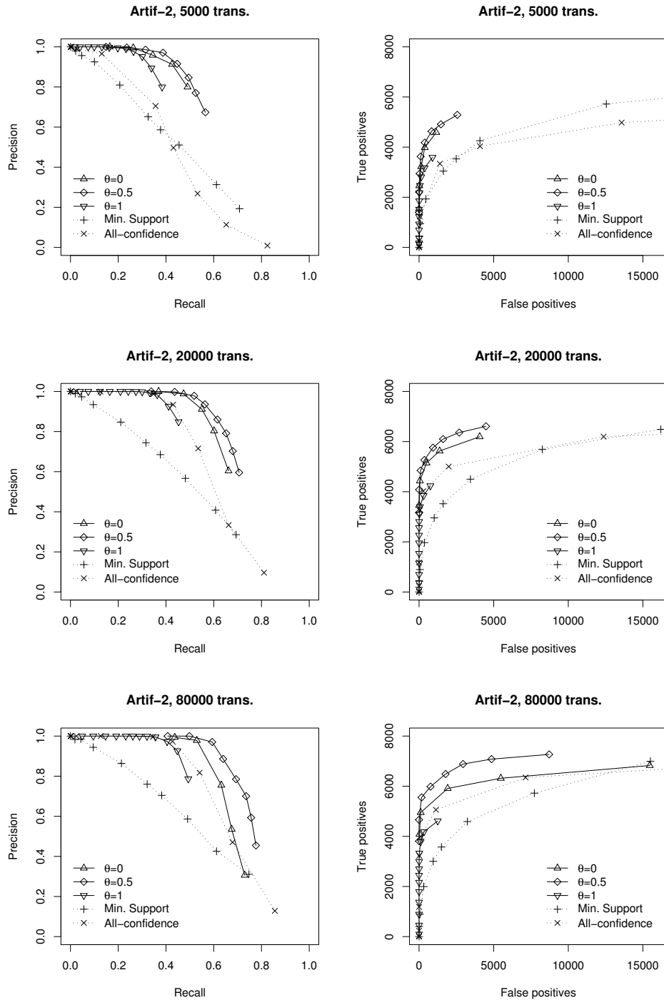
Figure 12: Performance of the algorithm on Artif-2 using different data set sizes.
